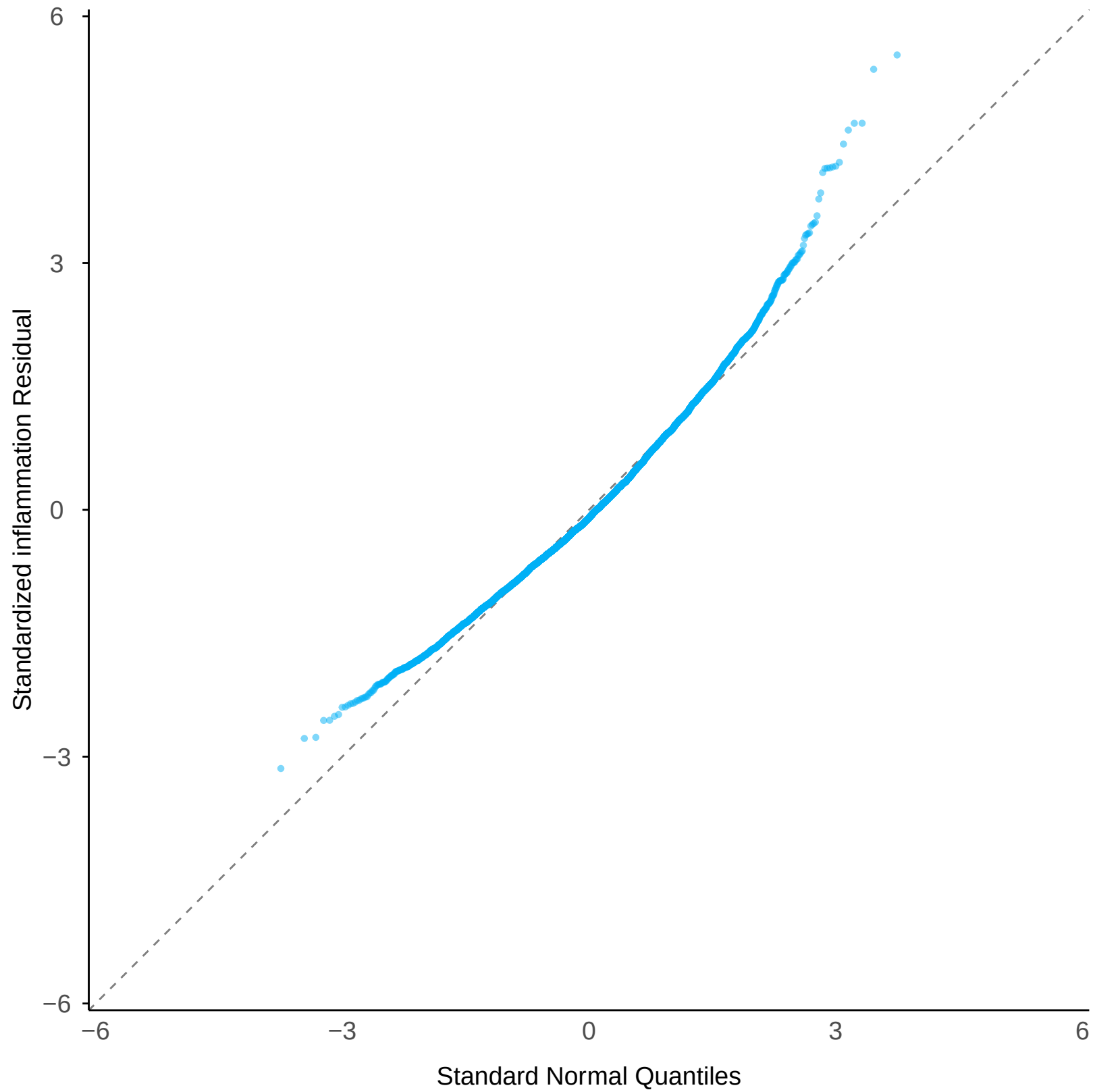
Normal Q-Q: inflammation Residual
