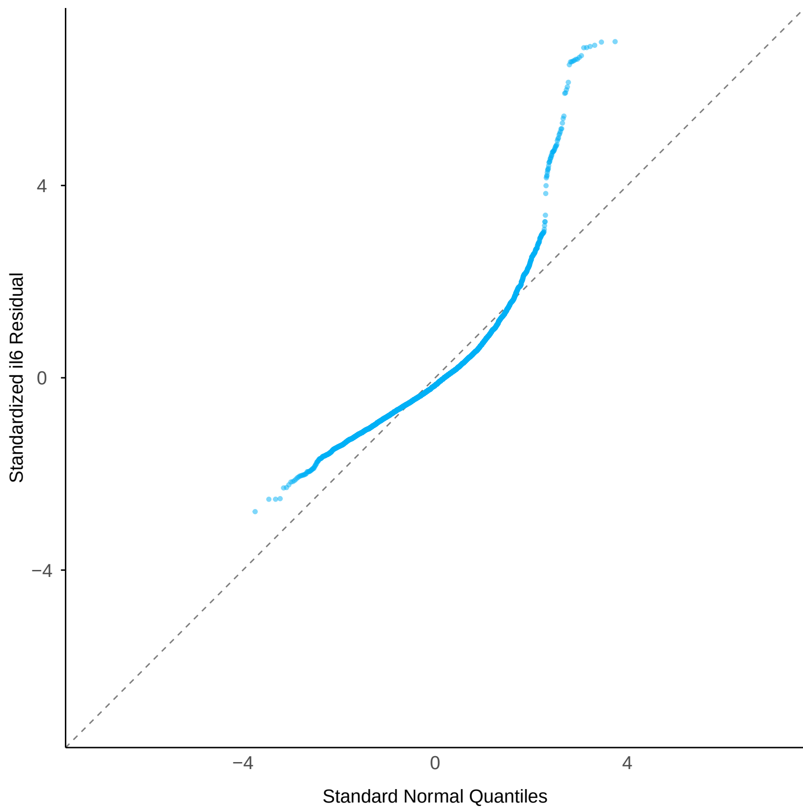
Normal Q-Q: il6 Residual
