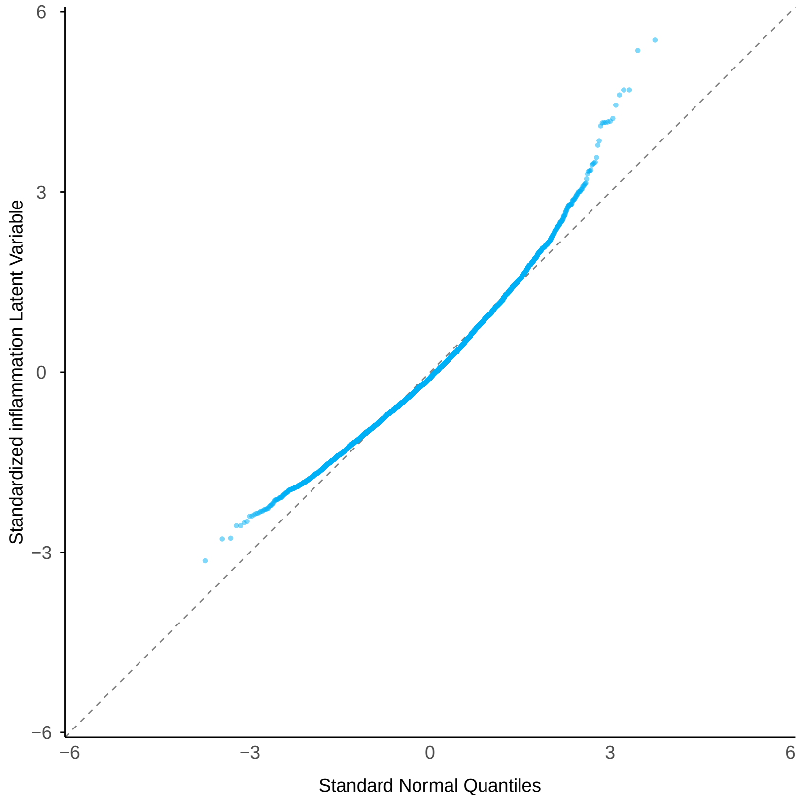
Normal Q-Q: inflammation Latent Variable
