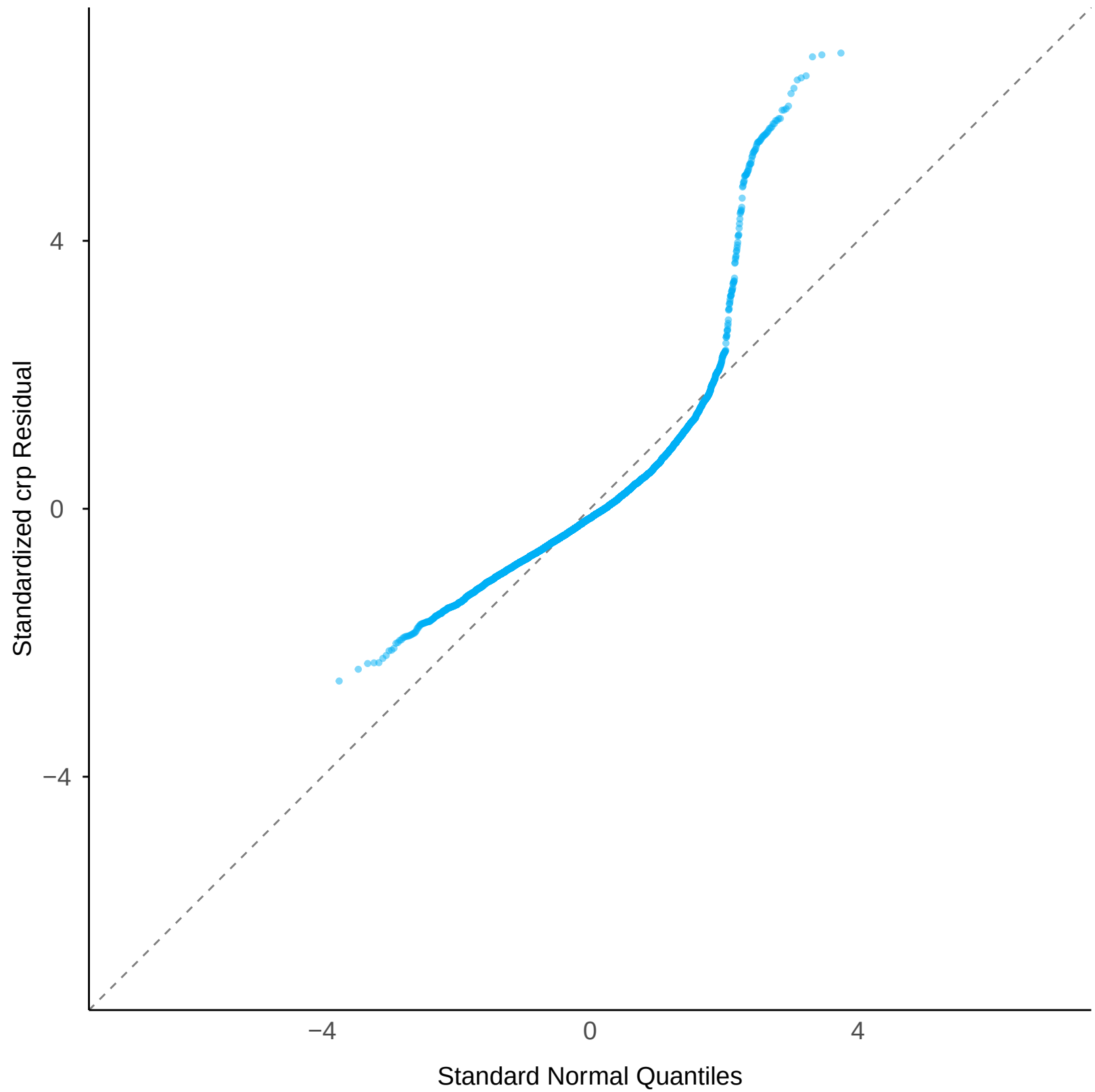
Normal Q-Q: crp Residual
