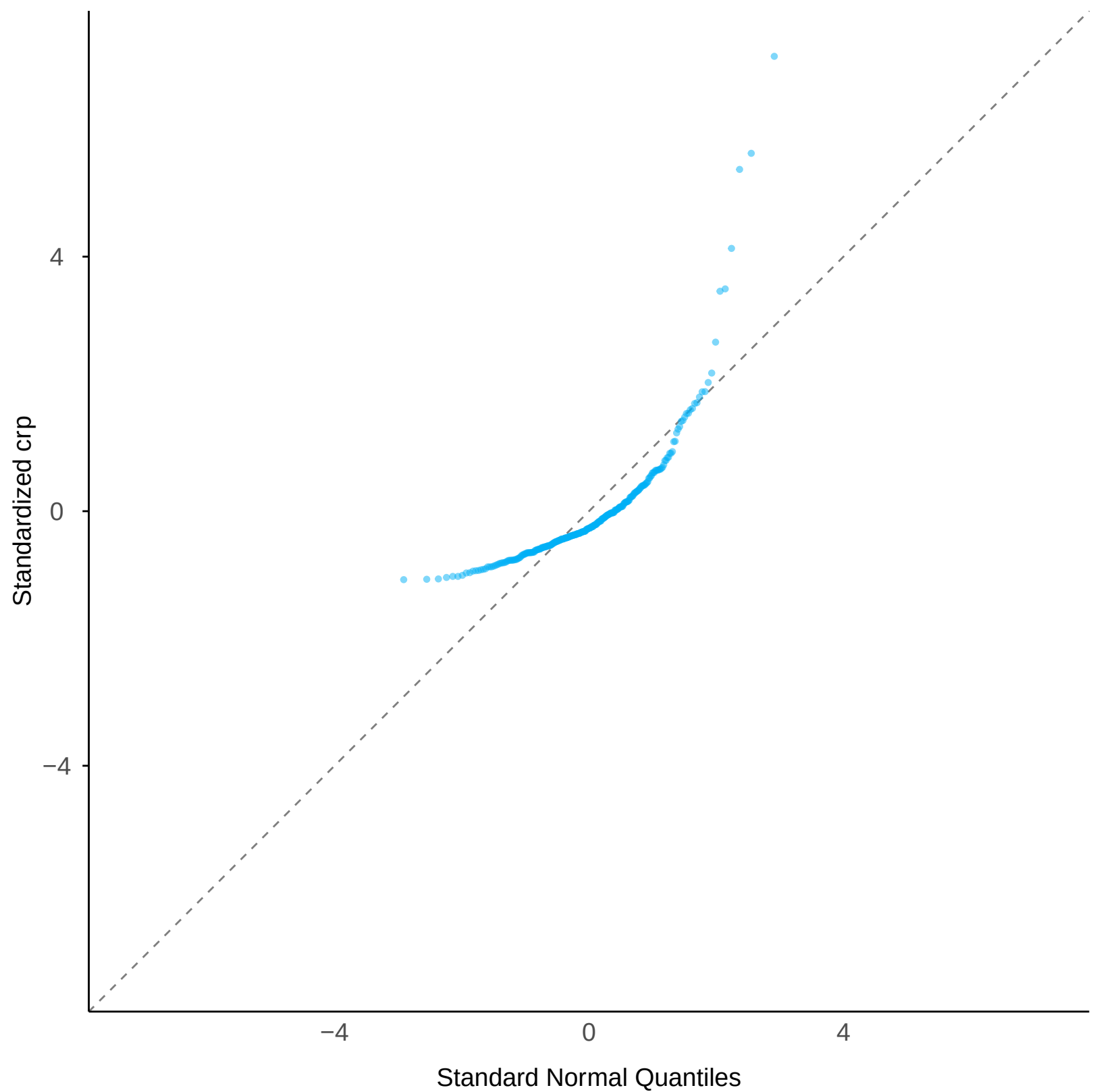
Normal Q-Q: crp
