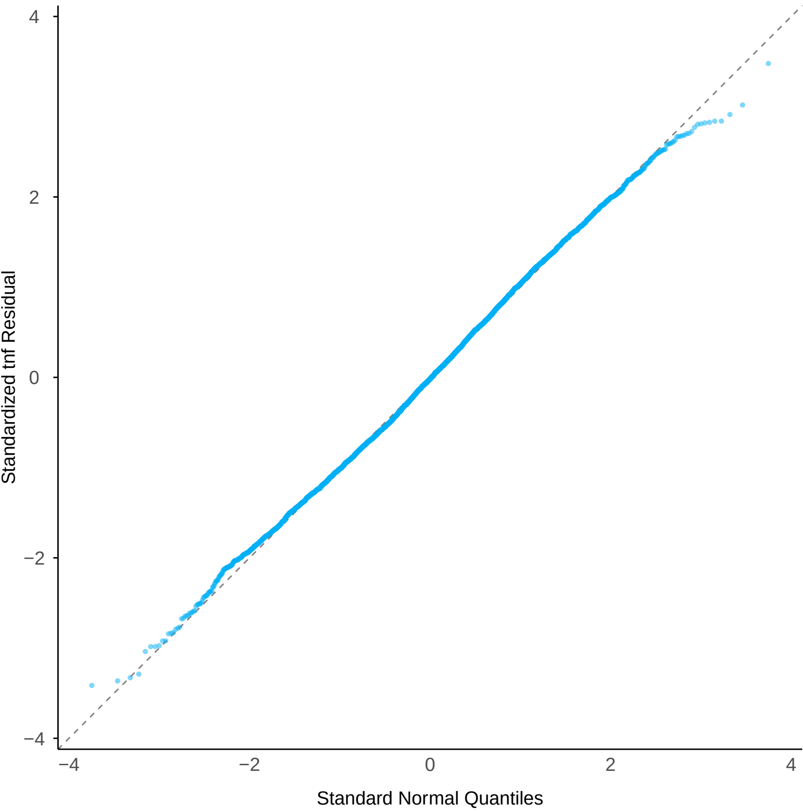
Normal Q-Q: tnf Residual
