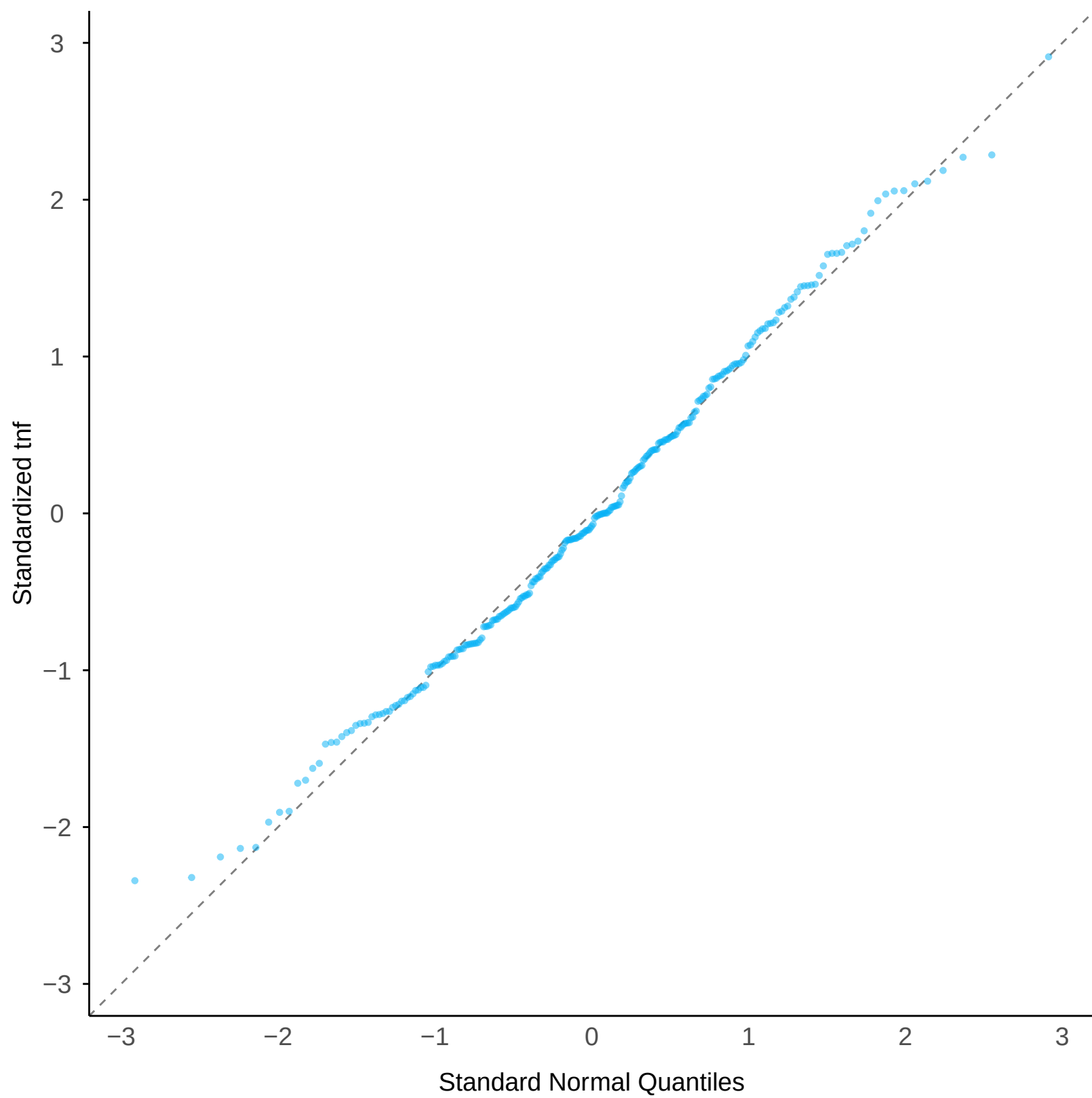
Normal Q-Q: tnf
