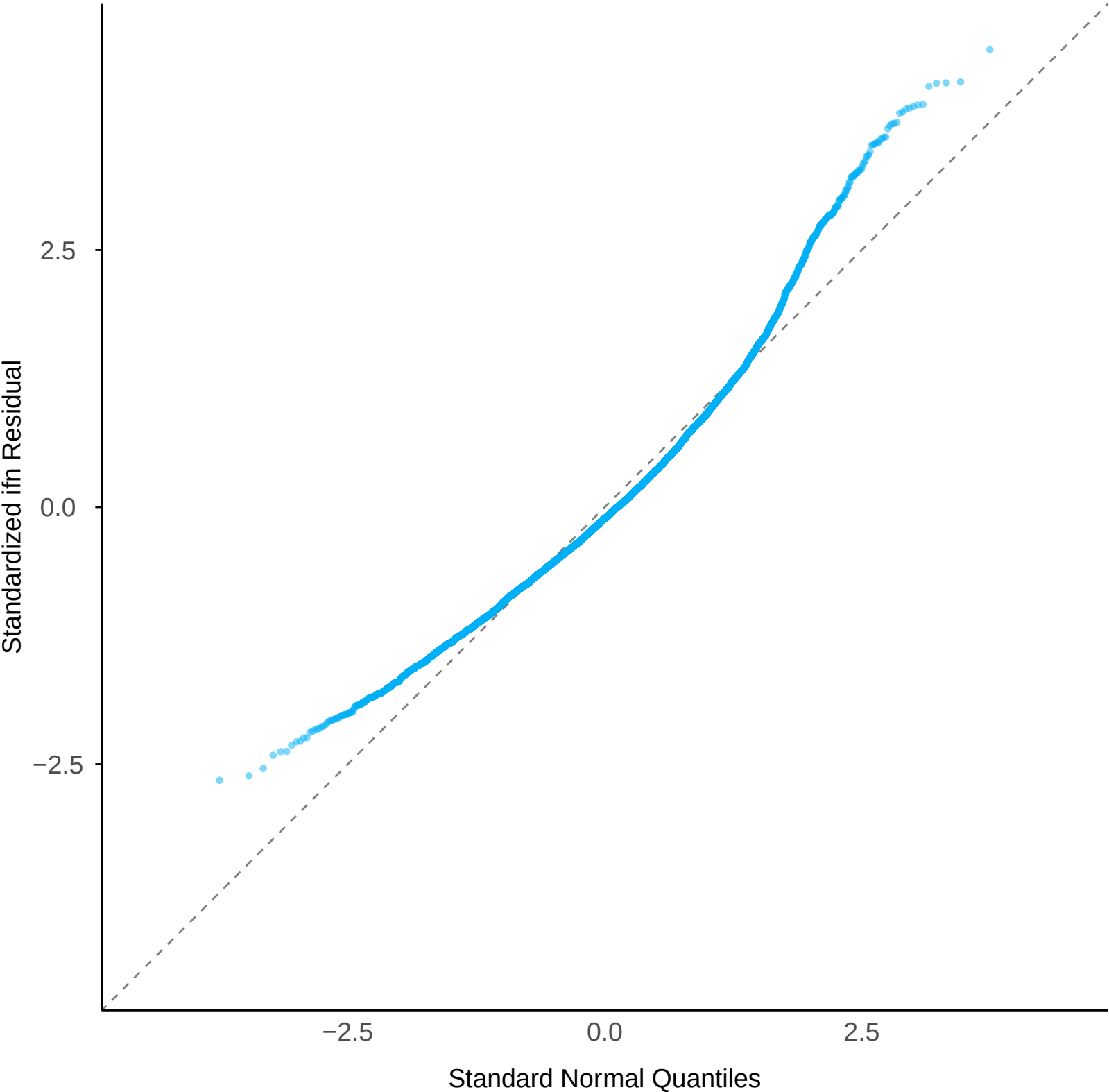
Normal Q-Q: ifn Residual
